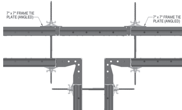
Typical T-Wall with Fillers
