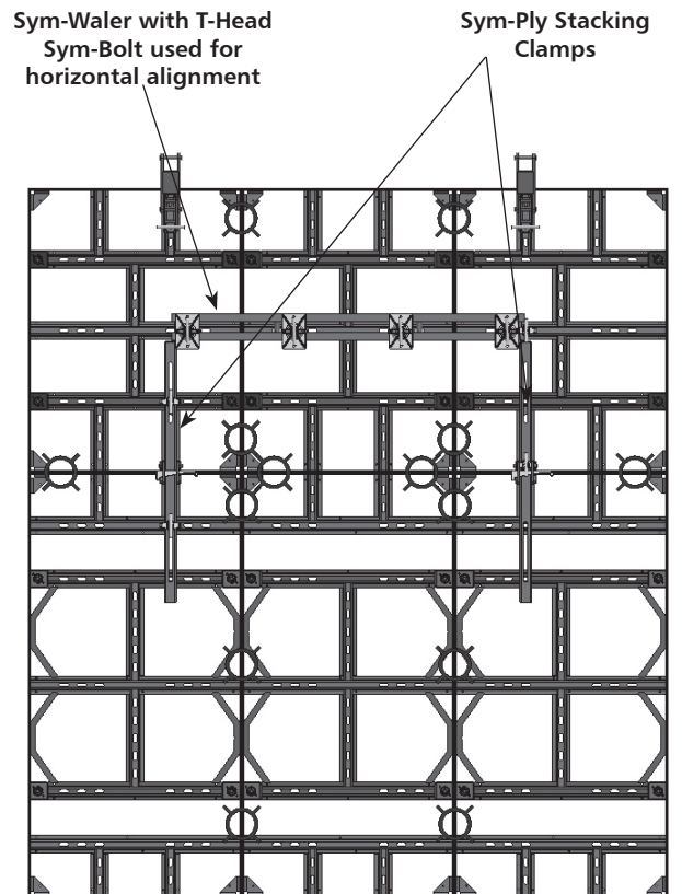
GANG — 3'-0" Wide x 6'-0" High + 4'-0" High x 3 Panels Wide
