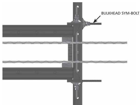
Typical Bulkhead with External Tie
