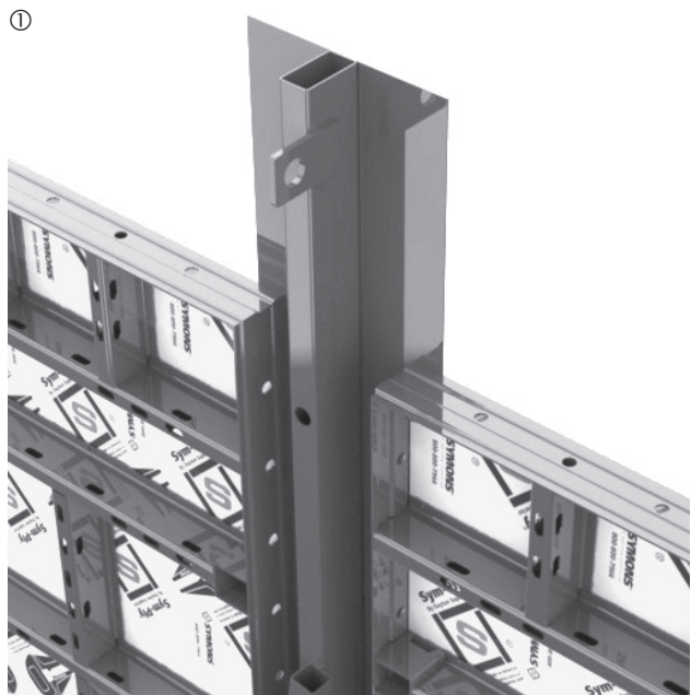
With gangs in position, lower the Slip Plate into position.
