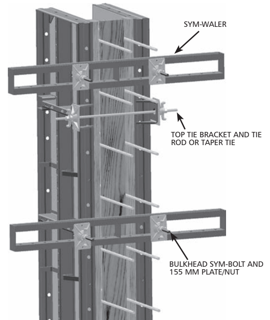
Typical Bulkhead with External Tie
