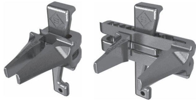
Sym-Clamp
