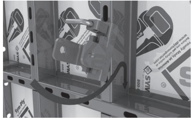
Aligner Bracket Installation
