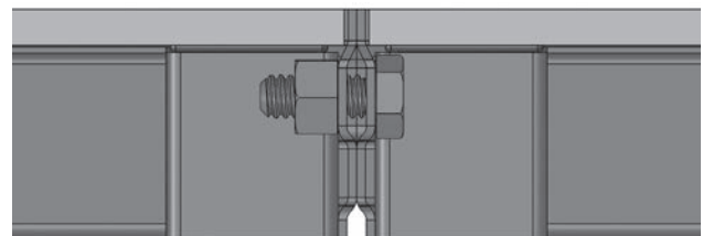
Typical Bolt Connection
