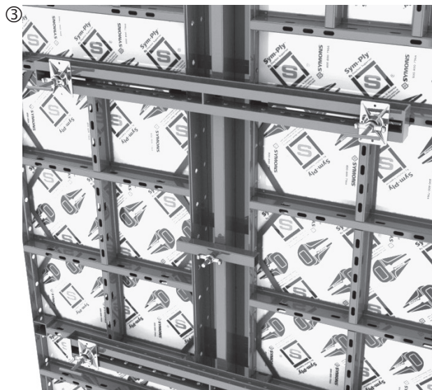
Add 60" Sym-Waler at tie locations.
