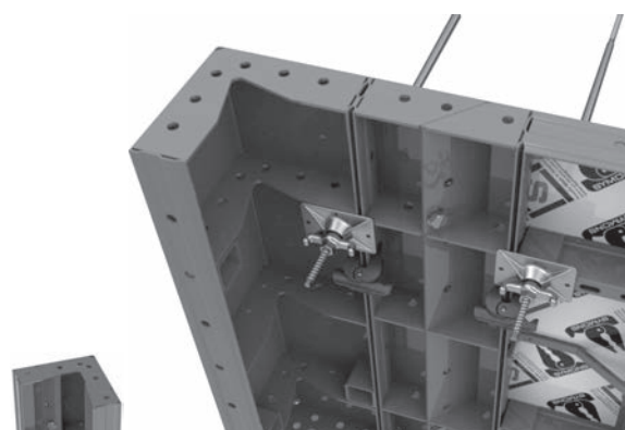
Stripping Panel
