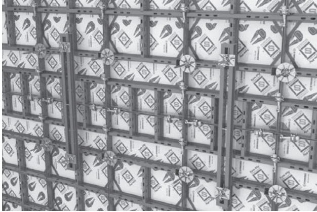
Stiffen Gangs with Sym-Waler (See Stacking Panels section for locations)
