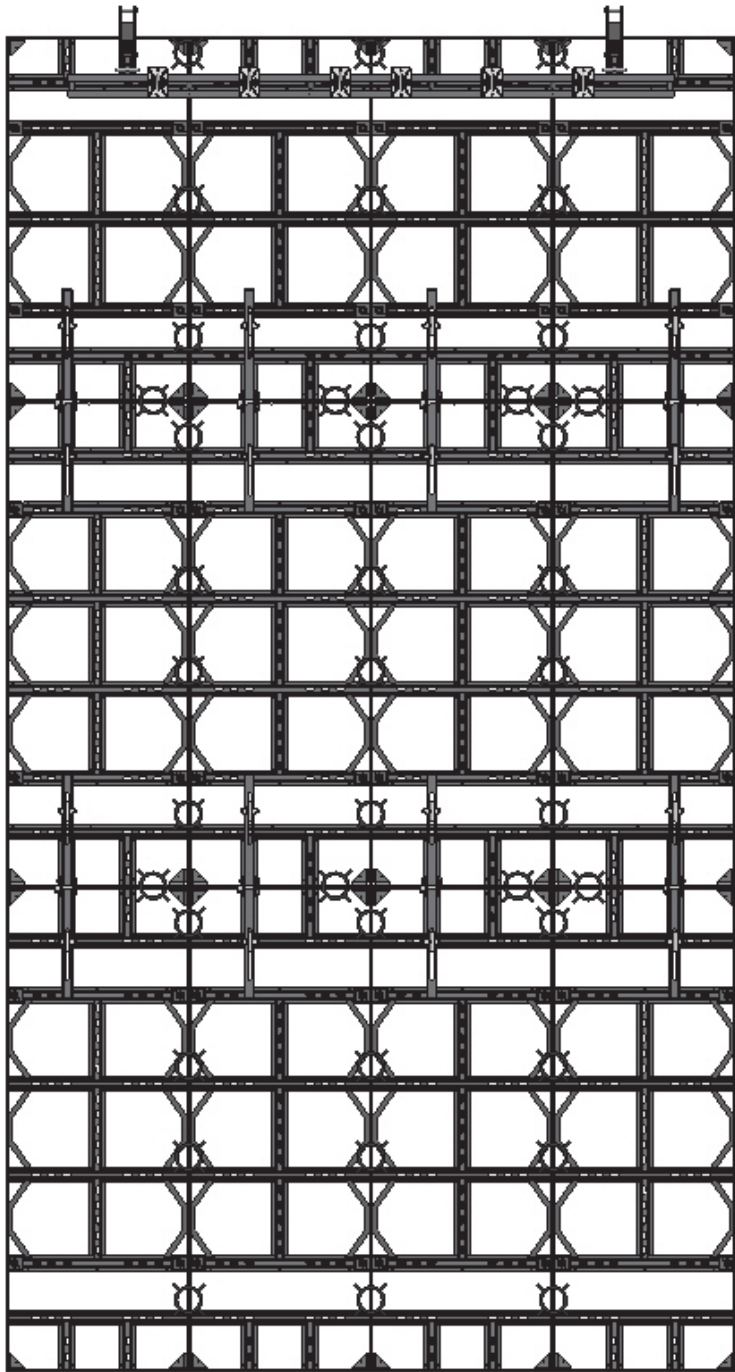
GANG — 3'-0" Wide x 8'-0" High + 8'-0" High + 6'-0" High x 4 Panels Wide
