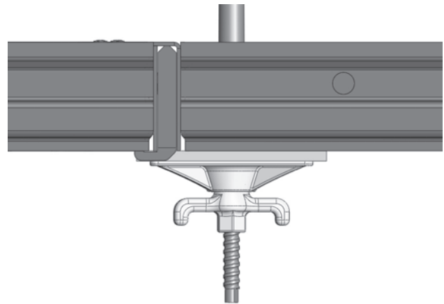
Typical Tie Placement Adjacent to 1" Filler
