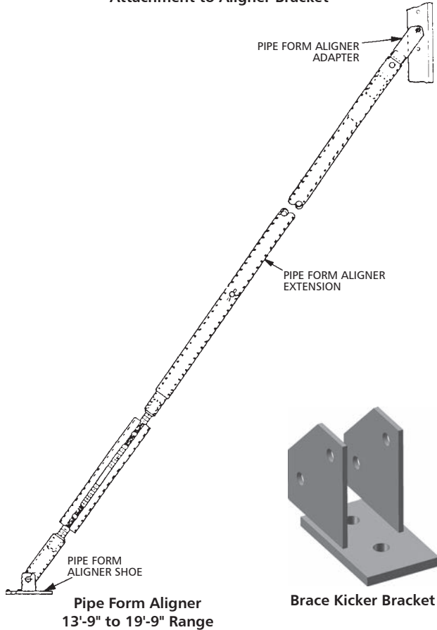
Attachment to Aligner Bracket
