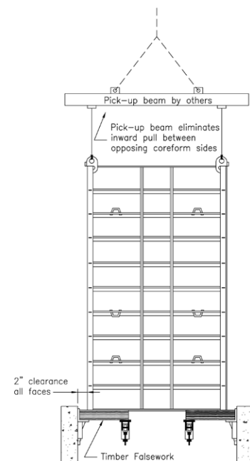
Cross Core Section Showing Lift Lines
