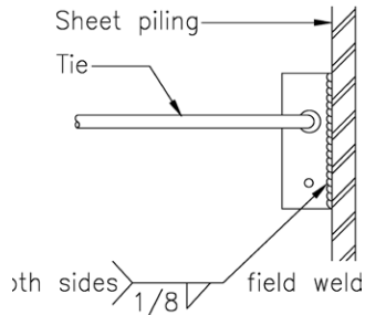
Single End Threaded Toggle Application #1
