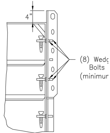
Column Lift Corner Installation
