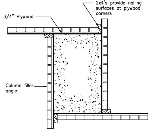
Typical "Run-By" Filler Angle Application
