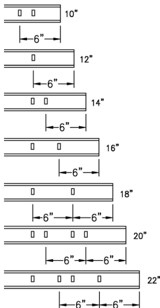
Slot Spacing for Filler End Rails
