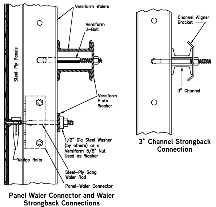
Section View
