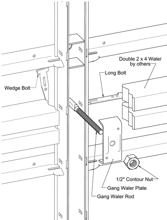
Gang Filler Double 2x4 Waler Attachment
