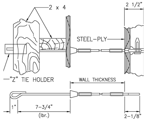
#2 Cone Tie
