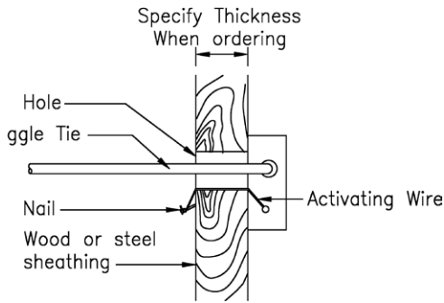
Single End Threaded Toggle Application #2
