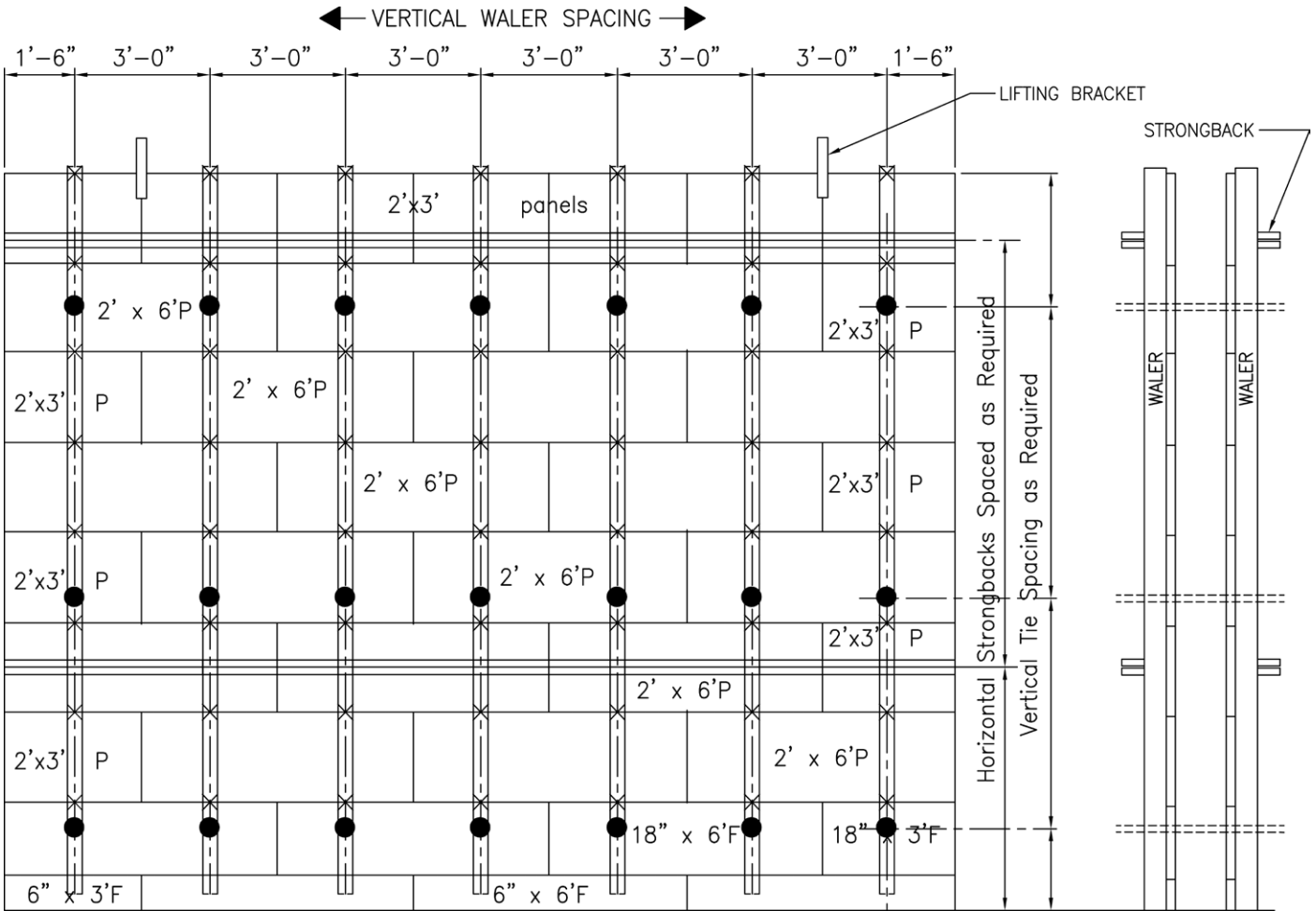
Horizontal Steel-Ply Waler Spacing
