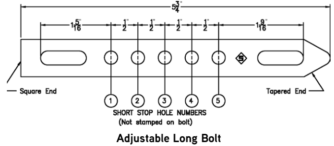
Adjustable Long Bolt
