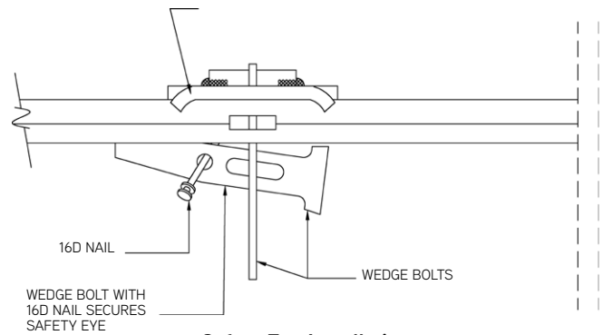
Safety Eye Installation
