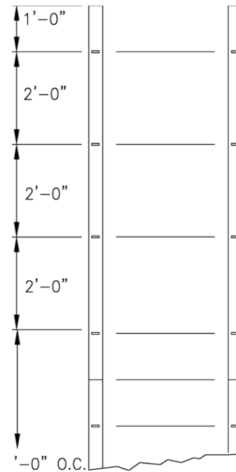
Tie Spacings Walls Taller Than 8' 6,000 lb Ultimate Tie Capacity
