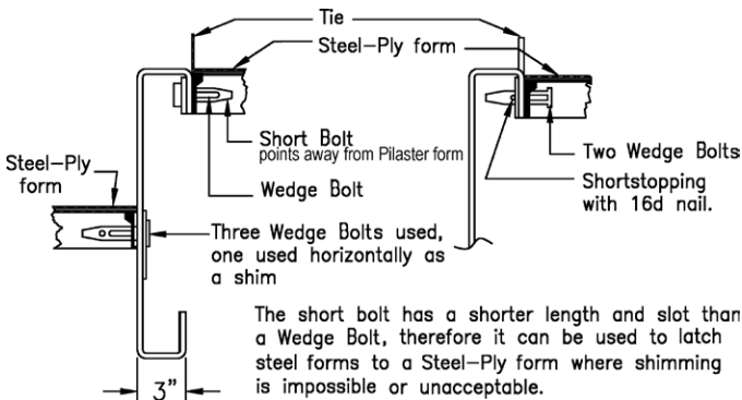
Short Bolt Short-Stopping and Shimming
