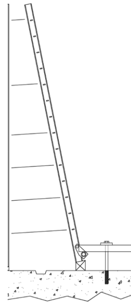
Battered Wall Tie Down
