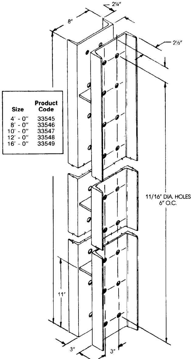
8" WALERS 8" Walers
