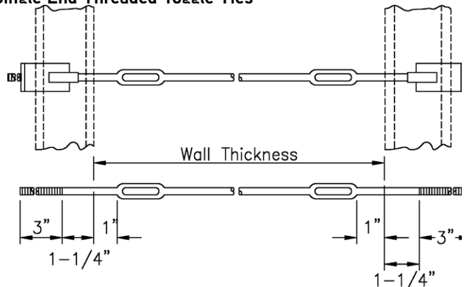
Tie Threaded Both Ends
