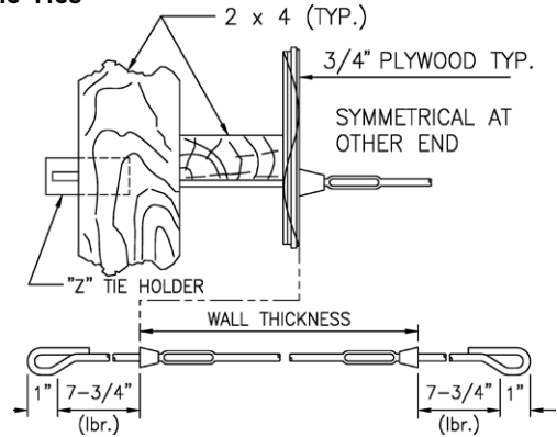
#1 Cone Tie
