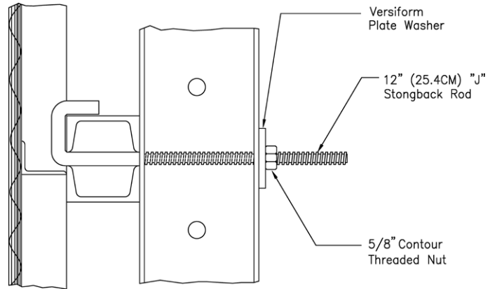
View B-B
