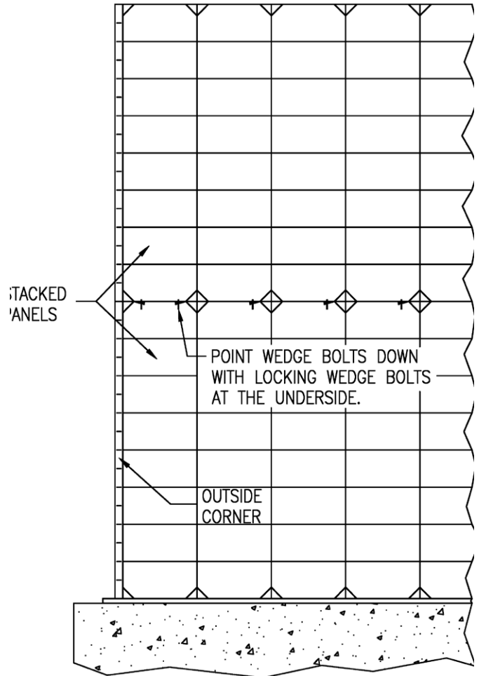
Typical Wedge Bolt Locations for Stacked Forms
