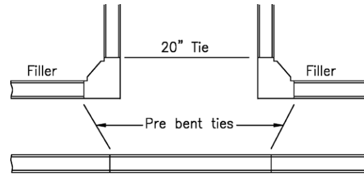
Pre-Bent Panel Tie Application for Intersecting Walls over 16"
