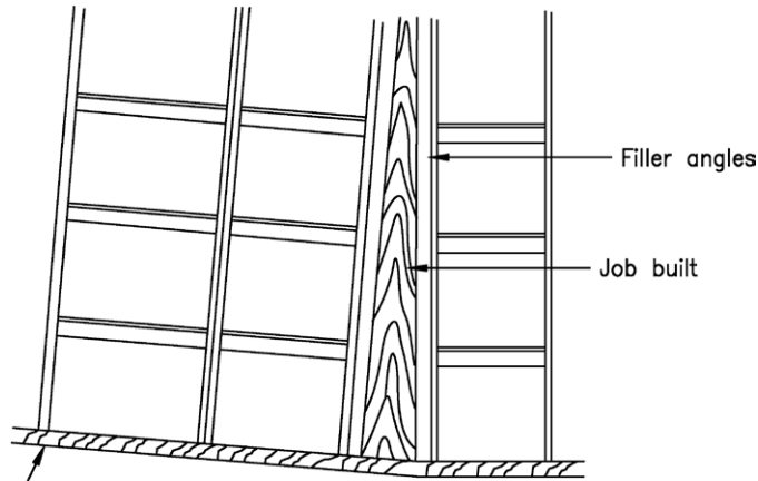
Typical Sloped Transition to Plumb Forms
