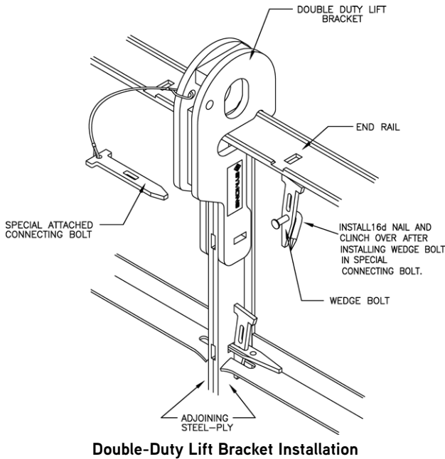
Double-Duty Lift Bracket Installation
