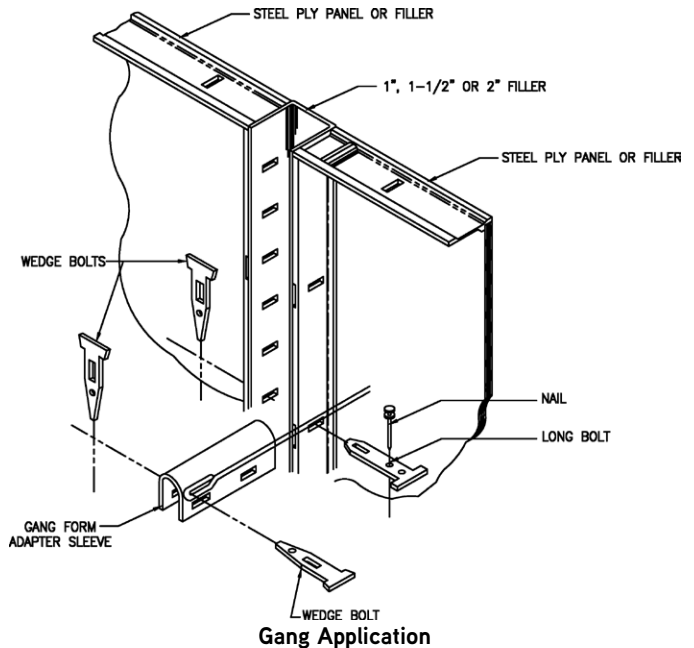
Gang Application
