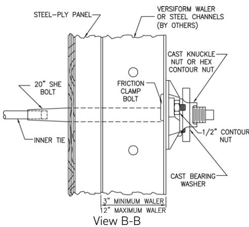
Cast Bearing Washer and She-Bolt Detail
